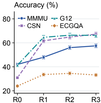
(a) MCQ accuracy
